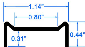
HPHTS & HPHRS Side View (Actual Size)
