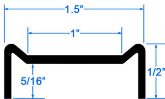
HPHTL & HPHRL Side View (Actual Size)
